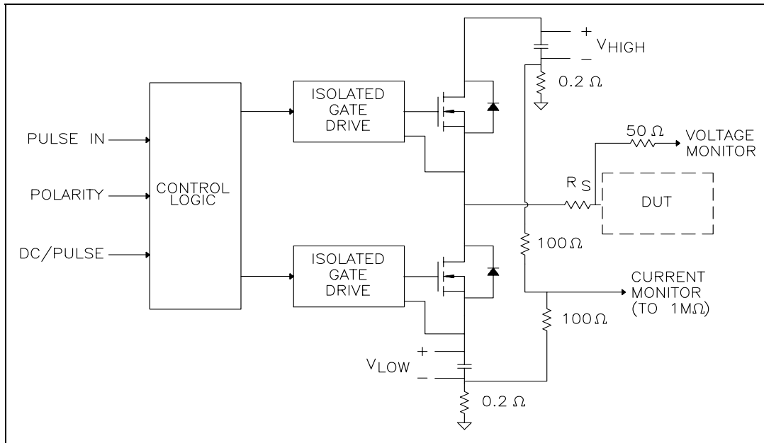
Figure 1. PVX-2505 Pulser functional schematic diagram
