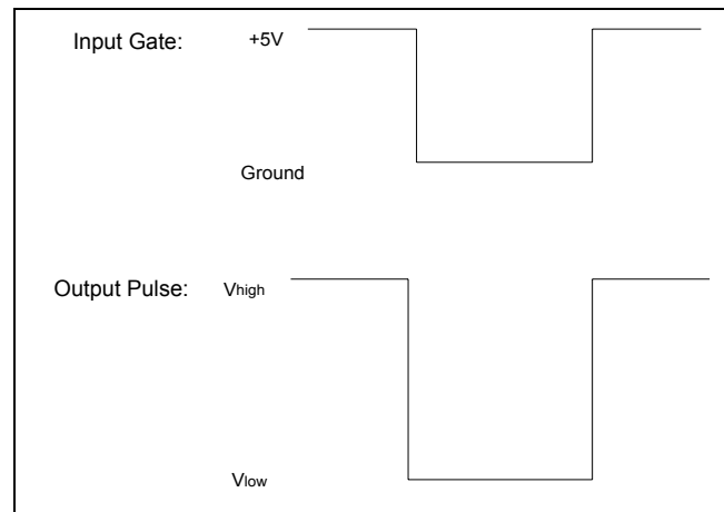
Generating a Negative Pulse With The PVM-4140
