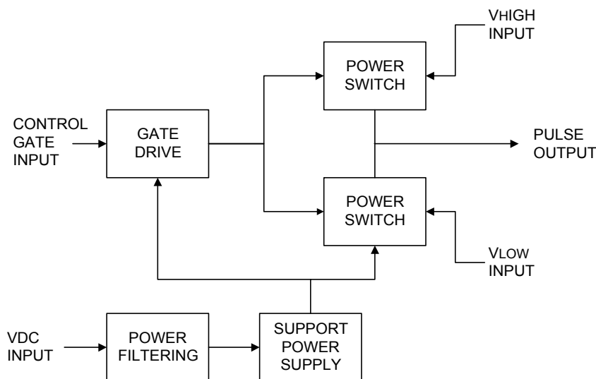
PVM-4140 Functional Block Diagram
