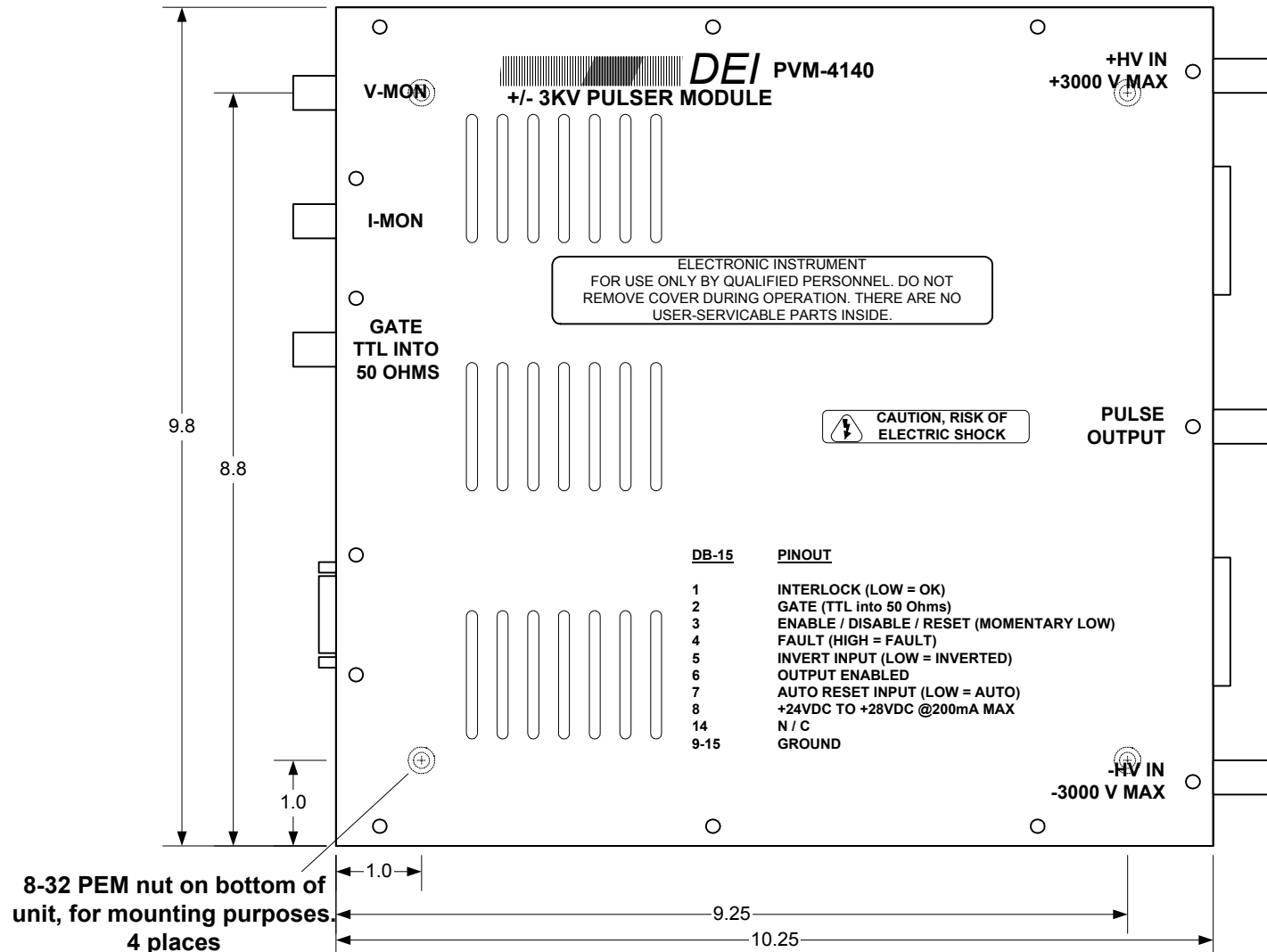
PVM-4140 Mechanical Dimensions And Mounting Hole/Connector Locations Not to scale. All dimensions are in inches
