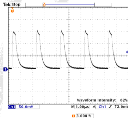
500KHz Frequency, 125A Output (1μs/Div horizontal scale, 50A/Div vertical scale)
