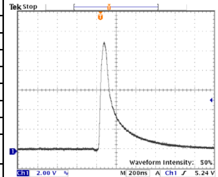
<100ns Minimum Pulse Width, 125A Output (400ns/Div horizontal scale, 38A/Div vertical scale, measured at the load)
