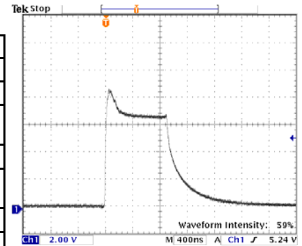
<30ns Rise Time, <750ns Fall Time, 120A Output (400ns/Div horizontal scale, 38A/Div vertical scale)
