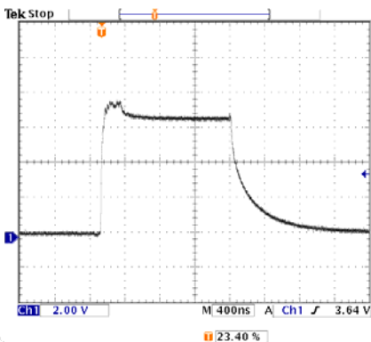
Typical Output Waveform 1.6μs Pulse Width, 125A Output (400ns/Div horizontal scale, 38A/Div vertical scale)
