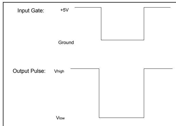
Generating a Negative Pulse With The GRX
